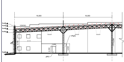
BUILDING SECTION
