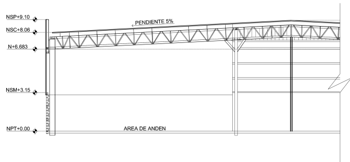
BUILDING SECTION
