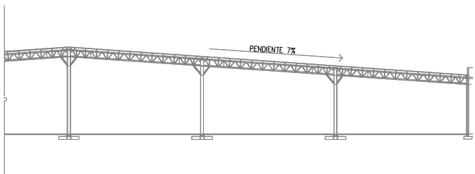
BUILDING SECTION
