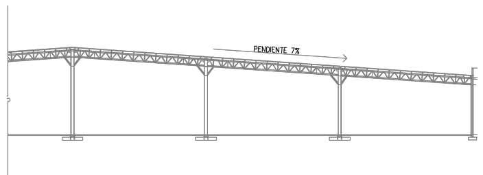
BUILDING SECTION
