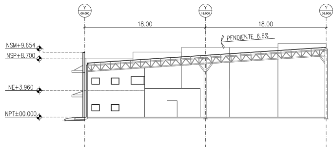
BUILDING SECTION
