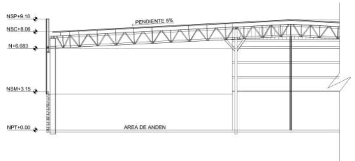
BUILDING SECTION
