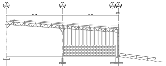
BUILDING SECTION
