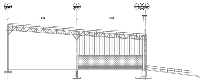
BUILDING SECTION
