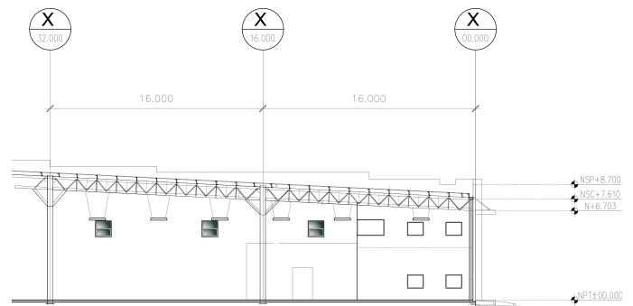
BUILDING SECTION
