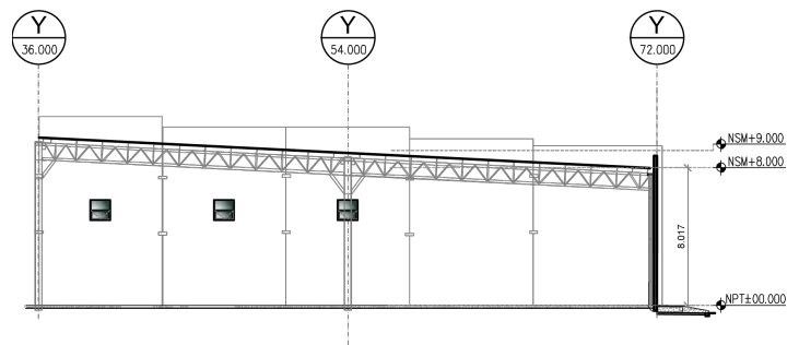
BUILDING SECTION
