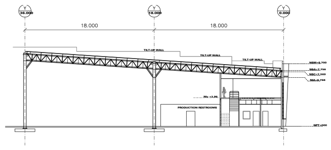
BUILDING SECTION
