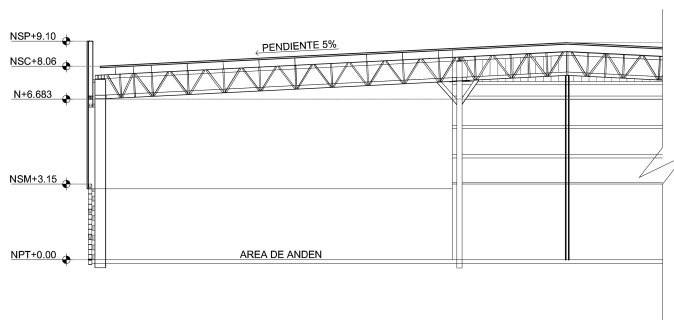
BUILDING SECTION
