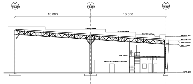
BUILDING SECTION
